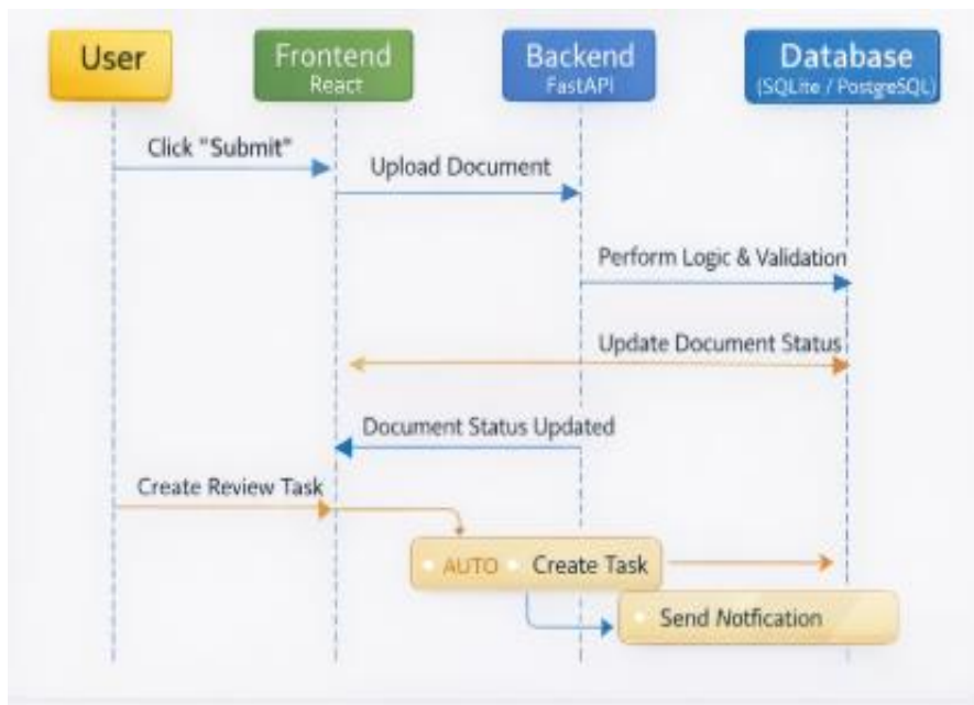
Figure 3: Sequence Diagram
